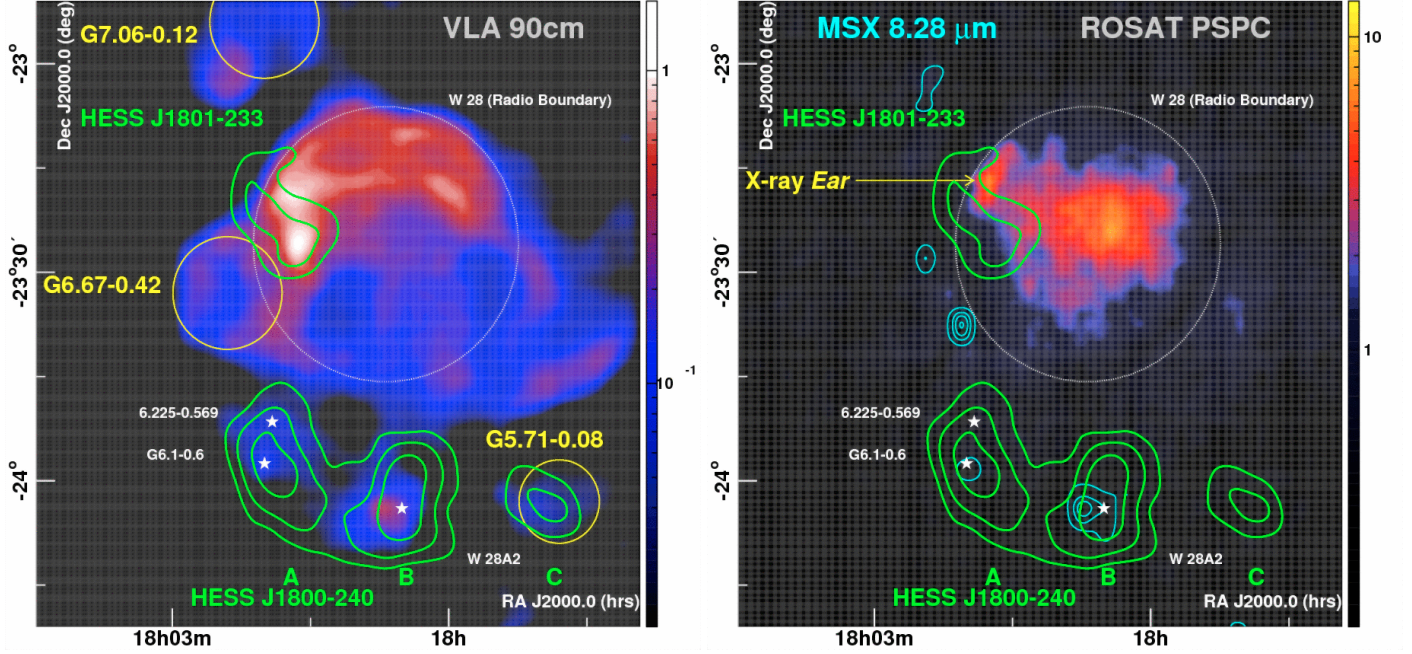
Fig. 3. Left: VLA 90 cm radio image from Brogan et al. (2006) in \text{Jy beam}^{-1} (rebinned by a factor 1.2 compared to the original). The VHE significance contours (green) from Fig. 1 are overlaid along with the HII regions (white stars) and the additional SNRs and SNR candidates (with yellow circles indicating their location and approximate dimensions) discussed in the text. Right: ROSAT PSPC image – 0.5 to 2.4 keV (smoothed counts per bin from Rho & Borkowski et al. 2002). Overlaid are contours (cyan – 10 linear levels up to 5 \times 10^{-4} \text{ W m}^{-2} \text{ sr}^{-1} ) from the MSX 8.28 \mu\text{m} image. Other contours and objects are as for the left panel . The X-ray Ear representing a peak at the northeastern edge is indicated.
