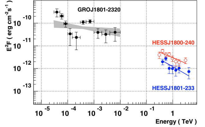
Fig. 4. Energy fluxes of HESS J1801–233 and HESS J1800–240 (for regions defined in Table 1) compared to the E > 100 MeV counterpart GRO J1801–2320. The power law fits and data points (summarised in Table 1) are also indicated: HESS J1801–233 (solid blue line and points); HESS J1800–240 (open red points and solid line); GRO J1801–232 (solid black points and grey 1\sigma confidence band).
