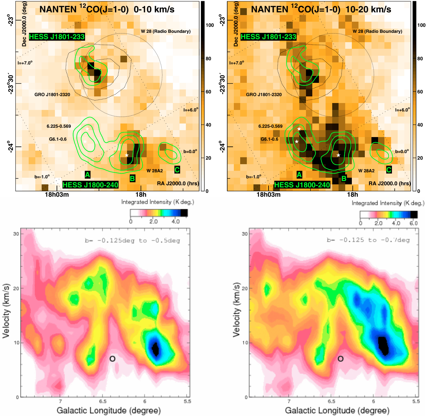
Fig. 2. Upper Left: NANTEN ^{12}\text{CO}(J = 1-0) image of the W 28 region (linear scale in K km s ^{-1} ) for V_{\text{LSR}} = 0 to 10 km s ^{-1} with VHE \gamma -ray significance contours overlaid (green) – levels 4, 5, 6\sigma as in Fig. 1. The radio boundary of W 28, The 68% and 95% location contours of GRO J1801–2320 and the location of the HII region W 28A2 (white stars) are indicated. Upper Right: NANTEN ^{12}\text{CO}(J = 1-0) image for V_{\text{LSR}} = 10 to 20 km s ^{-1} (linear scale and same maxima as for upper left panel). Bottom panels: distribution of CO emission over the Galactic longitude and V_{\text{LSR}} plane integrated over Galactic latitude b ranges -0.125^\circ to -0.5^\circ (left) and -0.125^\circ to -0.7^\circ (right). The latter range is used to show the effect of extending the latitude range to encompass component A of HESS J1800–240. The bold circle indicates the suggested systemic velocity (7 km s ^{-1} ) of W 28 from the HI studies of Velázquez et al. (2002).
