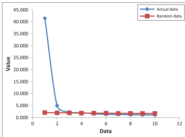
FIGURE 1: Scree and parallel analysis plot.
