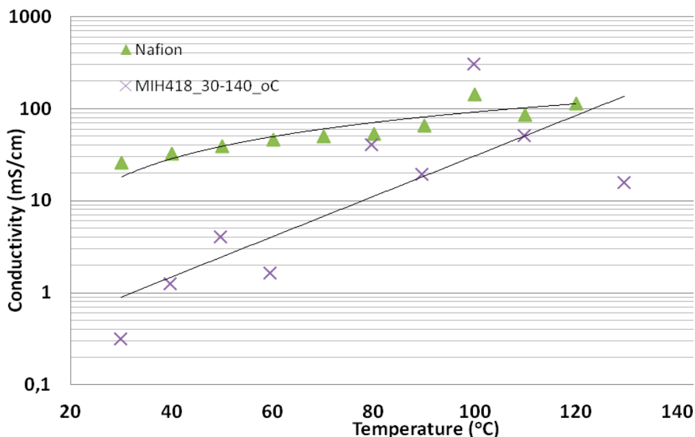
Figure 10. Proton conductivity of the acid excess acid-base blend membrane, relative humidity (RH) = 90% ± 4%, T = 30–130 °C.
