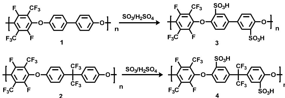
Scheme 2. Sulfonation products of poly(arylene ether perfluoroxylenes) (pPFX) 3 and 4 .
