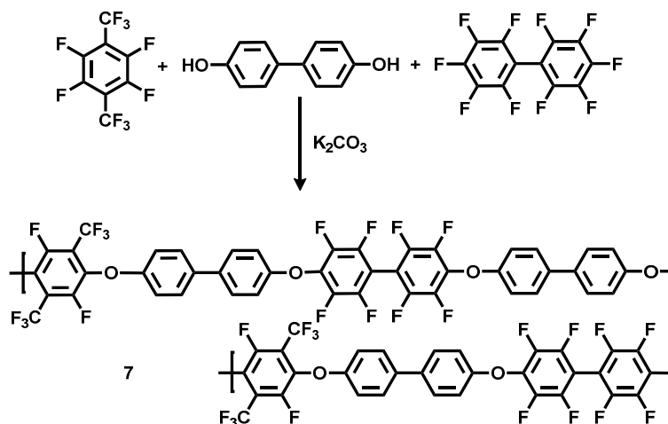
Scheme 5. Reaction scheme of the polycondensation reaction for the preparation of the statistical copolymer poly(aryleneetherperfluoroxylylene- co -decafluorobiphenyl) (pPFX-DBF) 7 .
