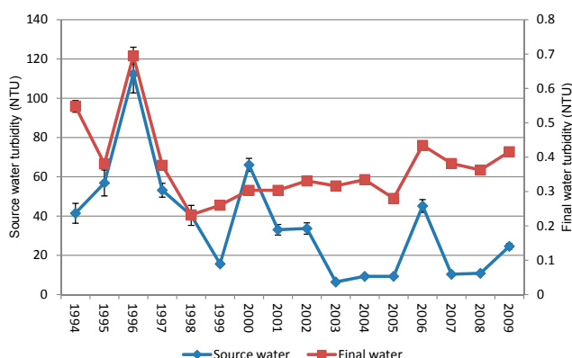
Figure 3 The average annual turbidity (NTU) of the source and final water from 1994 to 2009
