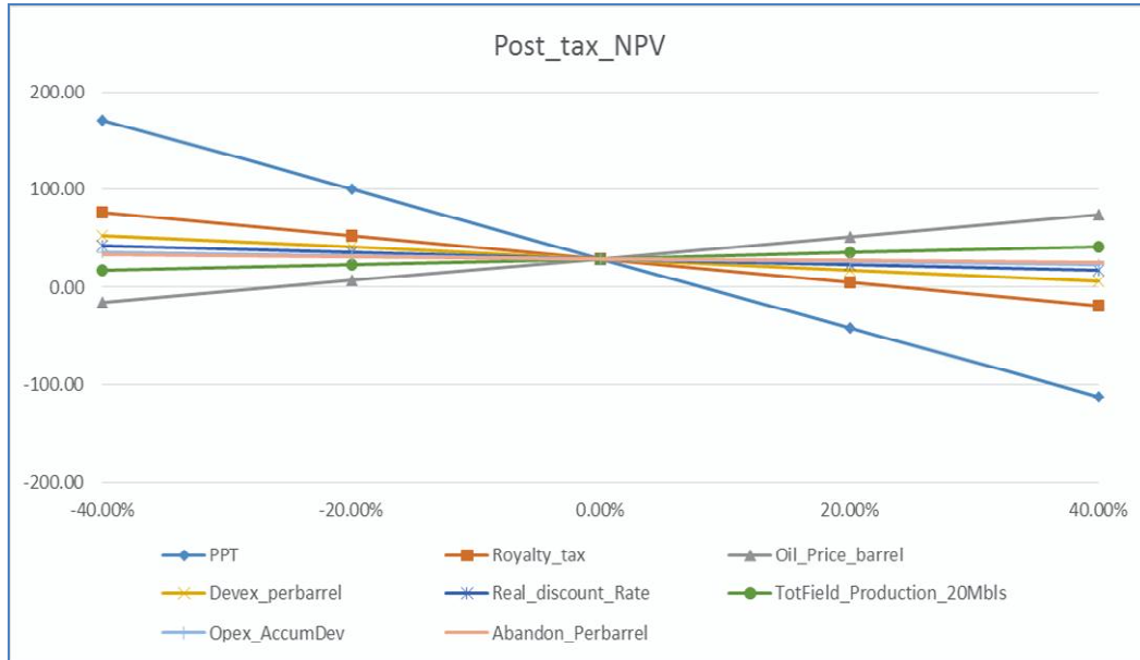
Figure 1: Spider chart measuring the effect of each parameter on field's NPV with the Steepness of the slope (Deviation of \pm 40\% using Crystal Ball)
