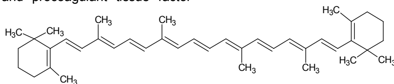
Figure 1: Structure of \beta -carotenes
