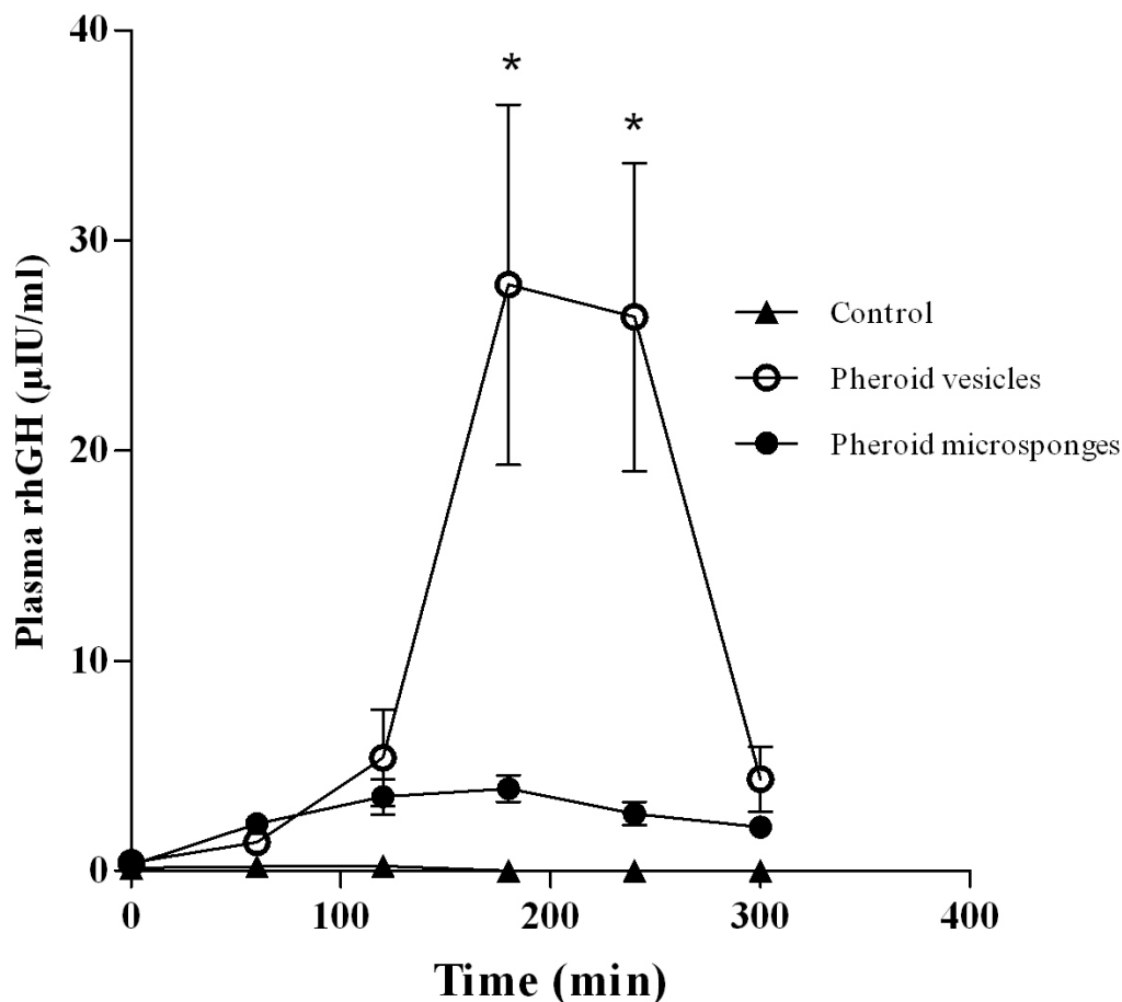
Figure 4. Plasma concentration-time profiles (300 minutes) of rhGH (3.6 IU/kg bodyweight) in a control, Pheroid vesicle and Pheroid microsphere formulations (mean \pm SD, n=4). The rhGH was entrapped in the Pheroid formulations for 24 h before nasal administration. *Statistically significant from the control and Pheroid microsponges, p < 0.05 .
