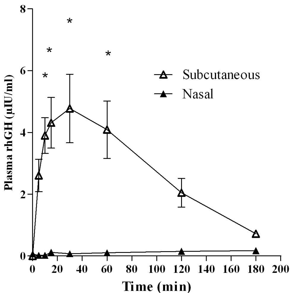
Figure 2. Concentration-time profile of rhGH in rat plasma obtained after subcutaneous injection of 0.6 IU/kg rhGH in physiological saline and after nasal administration of 3.6 IU/kg rhGH in physiological saline (mean \pm SD, n=6 ). *Statistically significant from the control (nasal) p<0.05 .
