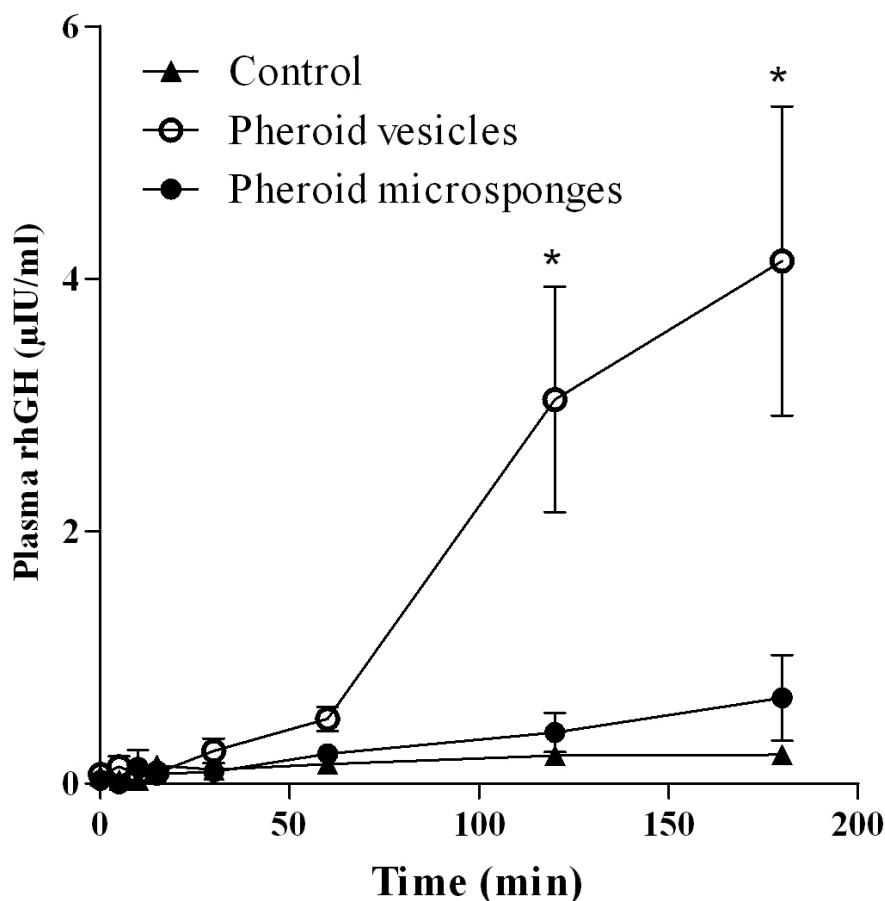
Figure 3. Plasma concentration-time profiles (180 minutes) of rhGH (3.6 IU/kg bodyweight) in a control, Pheroid vesicle and Pheroid microsphere formulations (mean \pm SD, n=6 ). The rhGH was entrapped in the Pheroid formulations for 30 minutes before nasal administration. *Statistically significant from the control and microspheres, p<0.05 .
