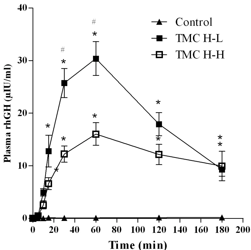
Figure 5. Plasma concentration-time profiles (180 minutes) of rhGH (3.6 IU/kg bodyweight) after nasal administration in the control, TMC H-H and TMC H-L formulations (mean \pm SD, n=6 ). *Statistically significant from the control, # from TMC-HH, p<0.05 .
