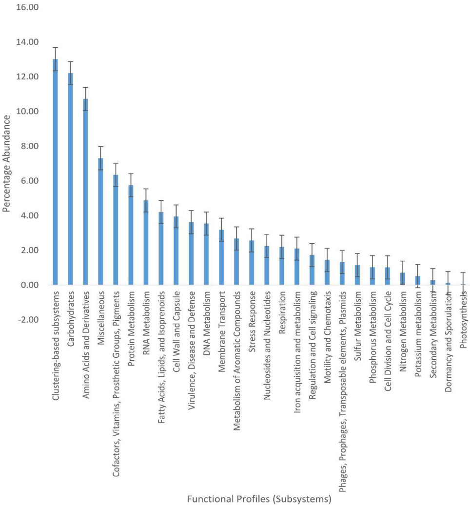
Fig. 2. Combined functional profiles of Congo cave soil microbiome dataset using SEED subsystem. Each bar represents the mean \pm standard error of each functional component recovered.
