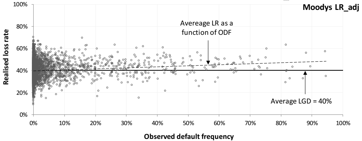
Figure 5. Original Moody's adjusted loss rates, using (3) with shock volatility Y_{TRR} = 0.2 .
