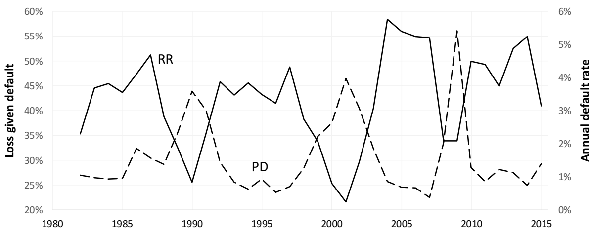
Figure 1. Global corporate default and recovery rates, 1983-2015.
