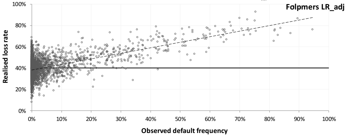
Figure 6. Folpmer's adjusted loss rates, using (5) with shock volatility Y_{r_{RR}} = 0.2 .
