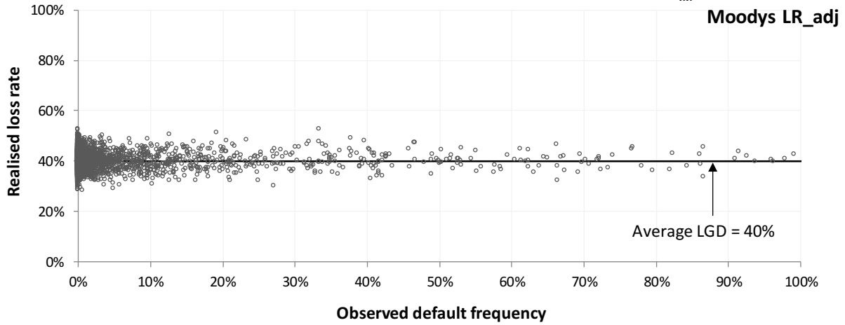
Figure 4. Moody's adjusted loss rates, using (3) – no shock volatility applied, i.e. Y_{TRR} = 0 .
