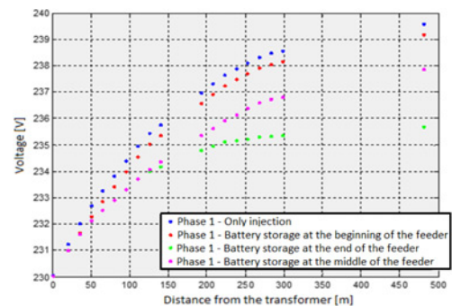
Fig. 7 Evaluation of storage location for an 30 kW PV system
