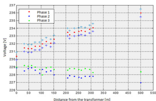
Fig. 6 Model validation – single-phase injection profile
