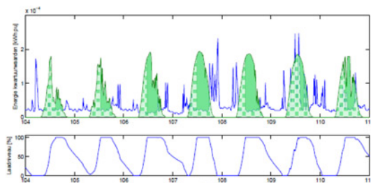
Fig. 2 Self-consumption for week 16, with an effective battery capacity of 1.5 kWh/MWh for an individual building
