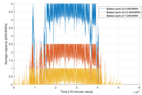
Fig. 3 Battery usage integrated in a residential household
