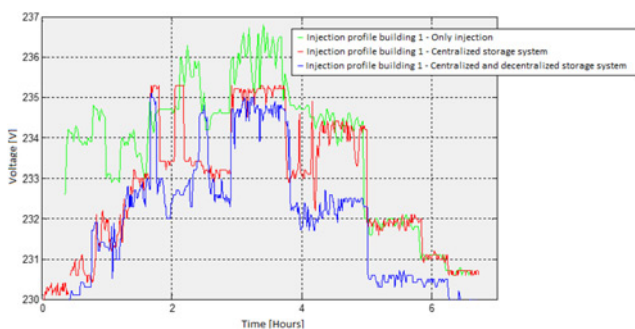
Fig. 10 Extra integration of decentralised storage system
