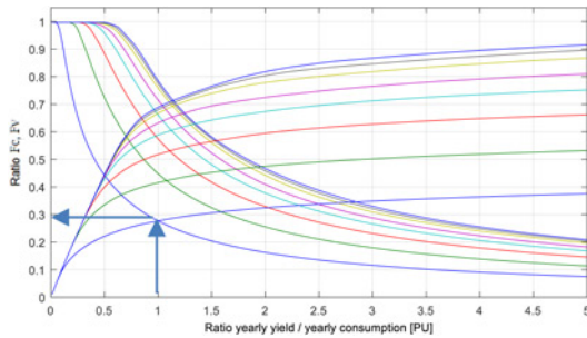
Fig. 1 F_C and F_V in function of the size of the PV installation for different effective storage capacities from 0 to 5 kWh/MWh with a cycle efficiency of 81% for an individual building
