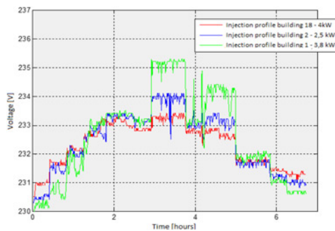
Fig. 9 Implementation of small centralised storage at the end of the feeder (building 1)
